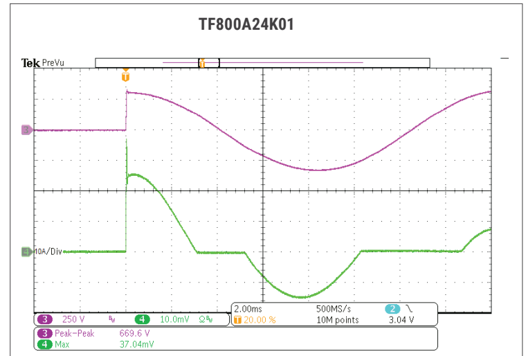
Fig. 08: INRUSH CURRENT AT 230VAC 800W.
