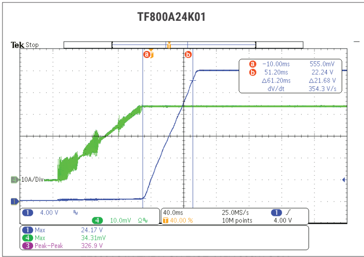
Fig. 11: TURN ON RISE TIME AT 115VAC 800W.
