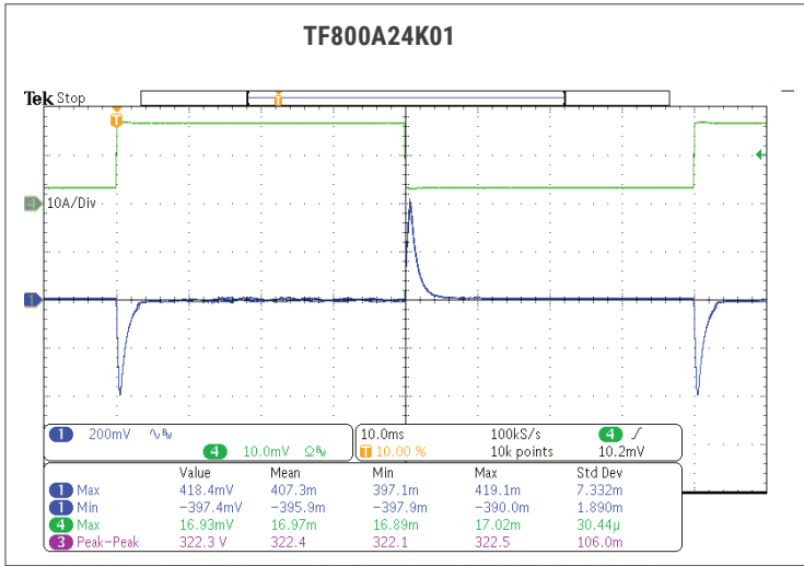
Fig. 26: TRANSIENT RESPONSE AT 115VAC, 10%-50% STEP LOAD.
