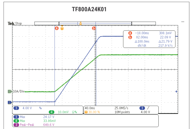
Fig. 14: TURN ON RISE TIME AT 230VAC 800W.
