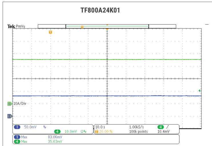
Fig. 23: SHORT CIRCUIT NO HCC-UP 230VAC.
