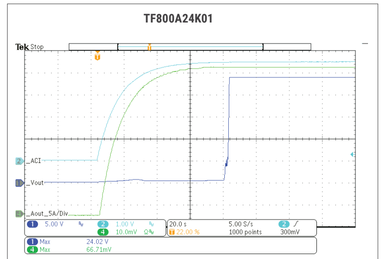
Fig. 39: LOCAL CURRENT PROGRAM (ACI) 230VAC.
