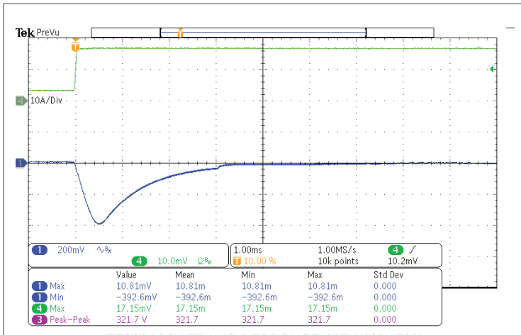
Fig. 28: TRANSIENT RESPONSE AT 115VAC, 10%-50% STEP LOAD.
