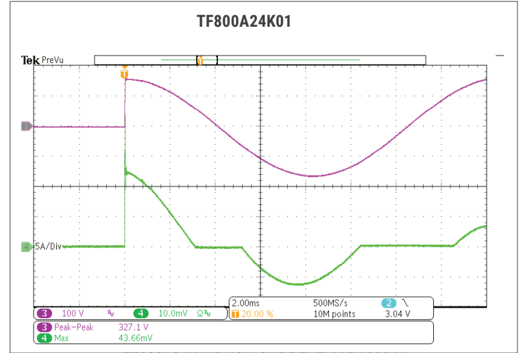
Fig. 06: INRUSH CURRENT AT 115VAC 800W.
