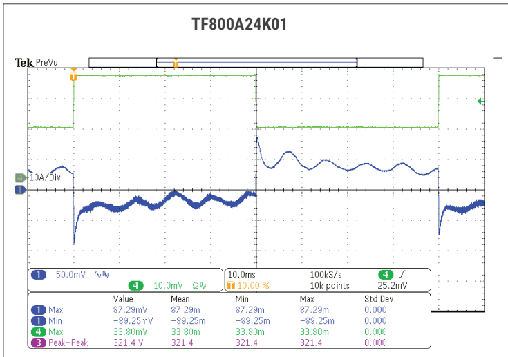
Fig. 32: TRANSIENT RESPONSE AT 115VAC, 50%-100% STEP LOAD.
