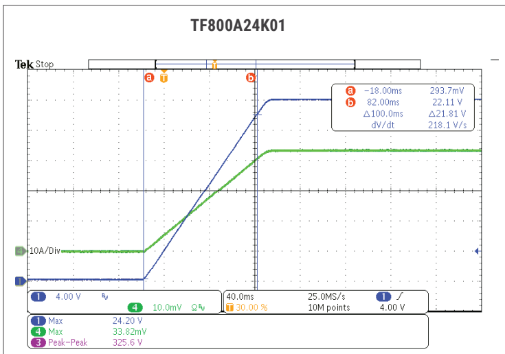
Fig. 13: TURN ON RISE TIME AT 115VAC 800W.
