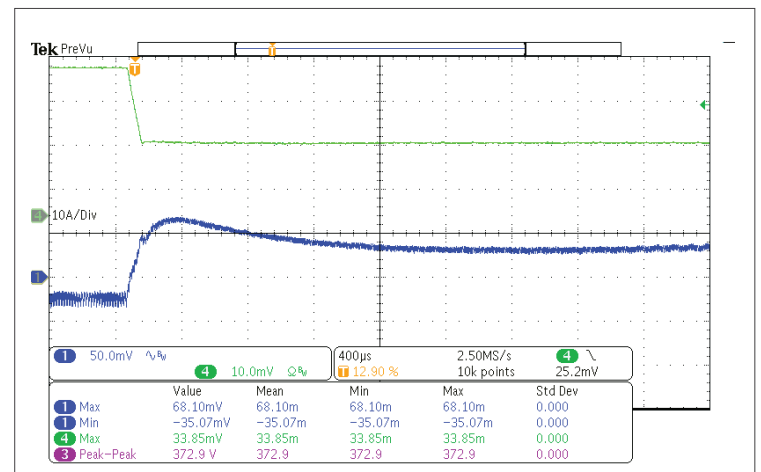
Fig. 37: TRANSIENT RESPONSE AT 230VAC, 50%-100% STEP LOAD.
