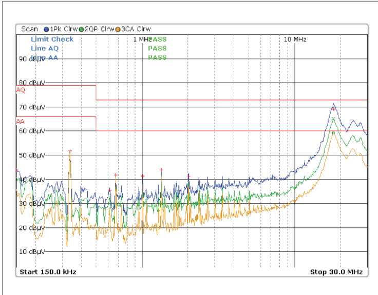
Fig. 68: CE Quasi Peak & Average 100% Load. 120V/60Hz Neutral.
