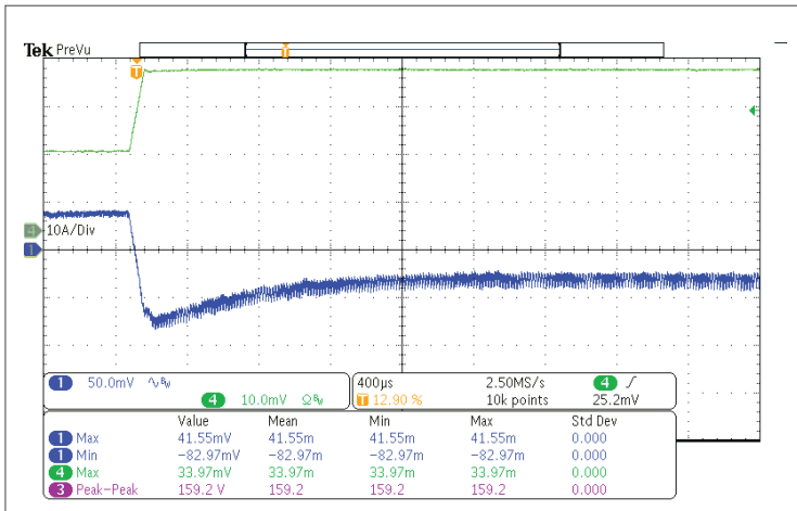
Fig. 34: TRANSIENT RESPONSE AT 115VAC, 50%-100% STEP LOAD.
