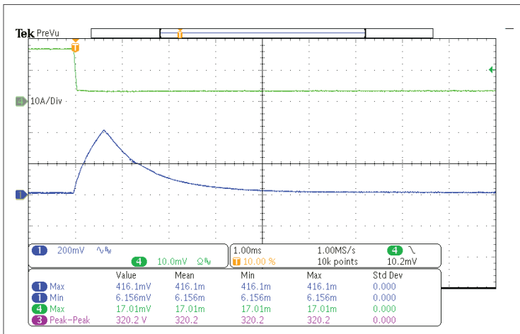
Fig. 30: TRANSIENT RESPONSE AT 115VAC, 10%-50% STEP LOAD.
