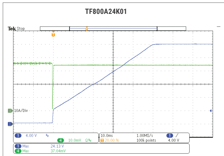
Fig. 25: SHORT CIRCUIT RECOVERY 230VAC.
