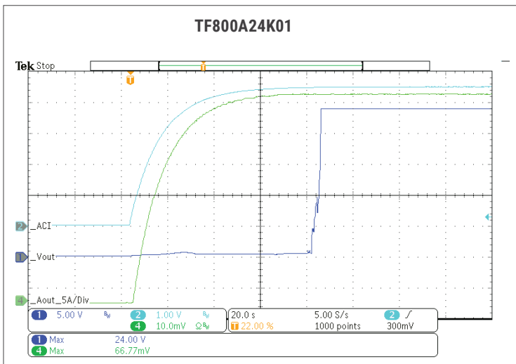
Fig. 38: LOCAL CURRENT PROGRAM (ACI) 115VAC.
