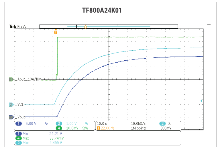
Fig. 47: LOCAL VOLTS PROGRAM (ACI) 230VAC.
