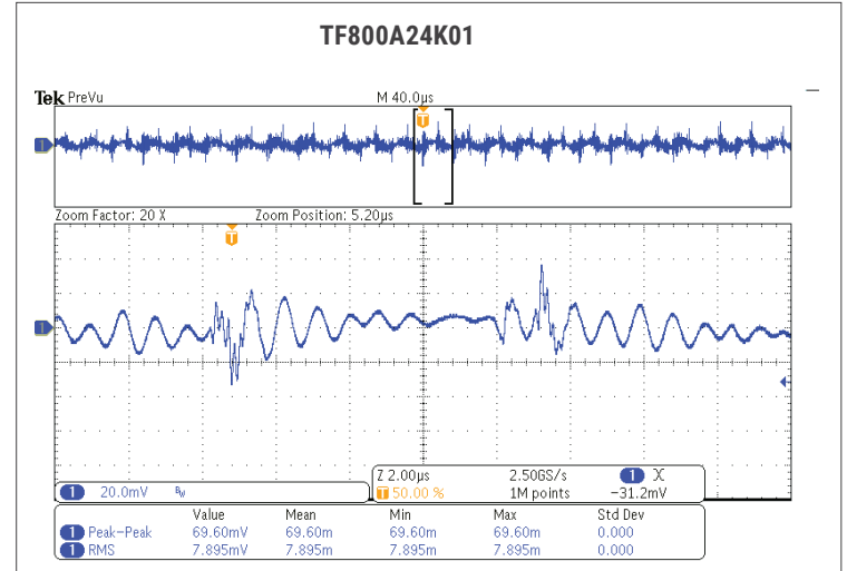
Fig. 69: CURRENT CM NOISE 230VAC 800W.
