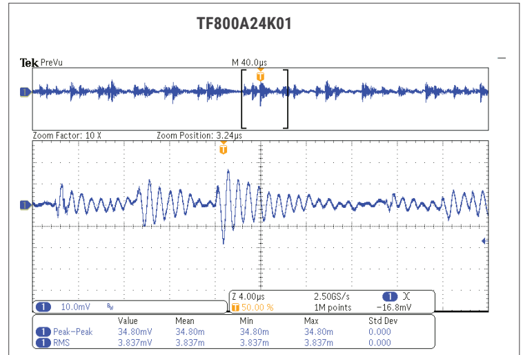
Fig. 67: CURRENT CM NOISE 230VAC 000W.
