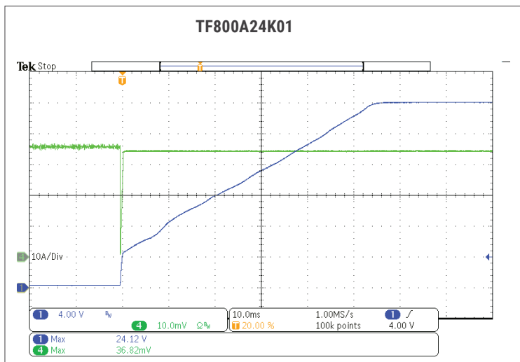
Fig. 24: SHORT RECOVERY 115VAC.
