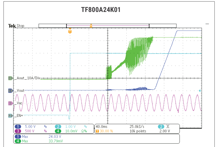
Fig. 55: INHIBIT (EN+)Hi Vout On 230VAC.
