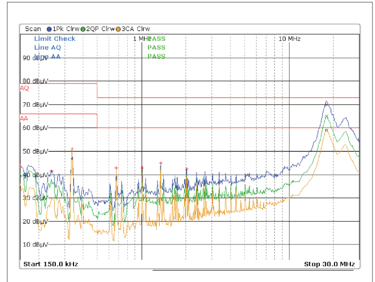
Fig. 67: CE Quasi Peak & Average 100% Load. 240V/60Hz Line.
