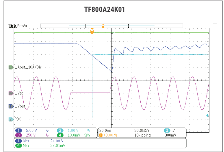
Fig. 65: POWER OK (POK) 230VAC 640W.
