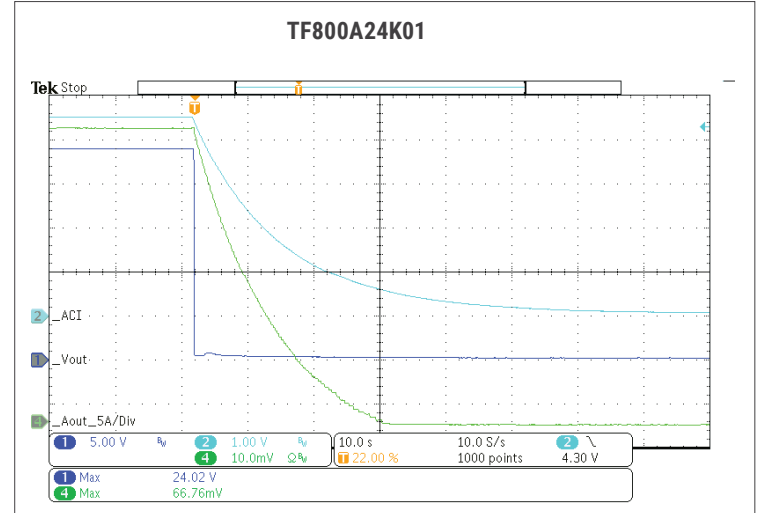
Fig. 41: LOCAL CURRENT PROGRAM (ACI) 230VAC.
