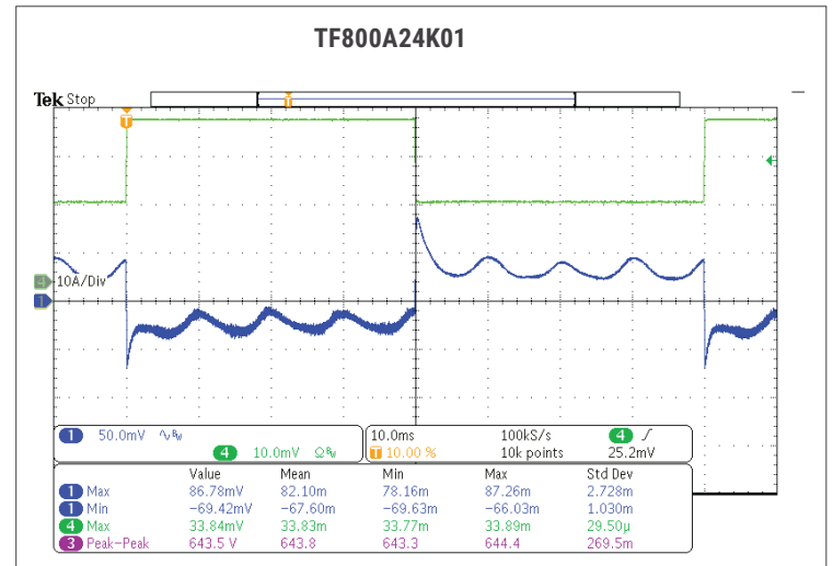
Fig. 33: TRANSIENT RESPONSE AT 230VAC, 50%-100% STEP LOAD.
