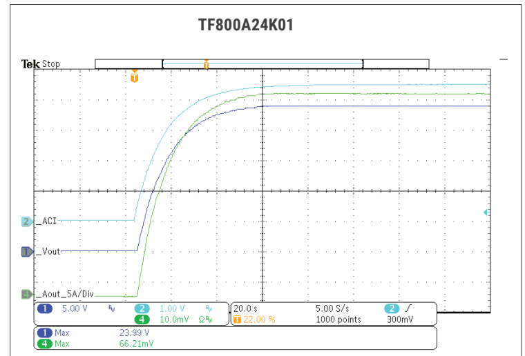
Fig. 43: LOCAL CURRENT PROGRAM (ACI) 230VAC.
