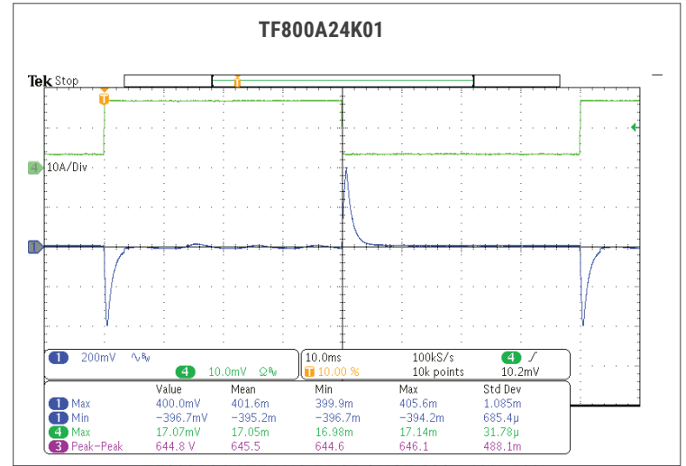
Fig. 27: TRANSIENT RESPONSE AT 230VAC, 10%-50% STEP LOAD.
