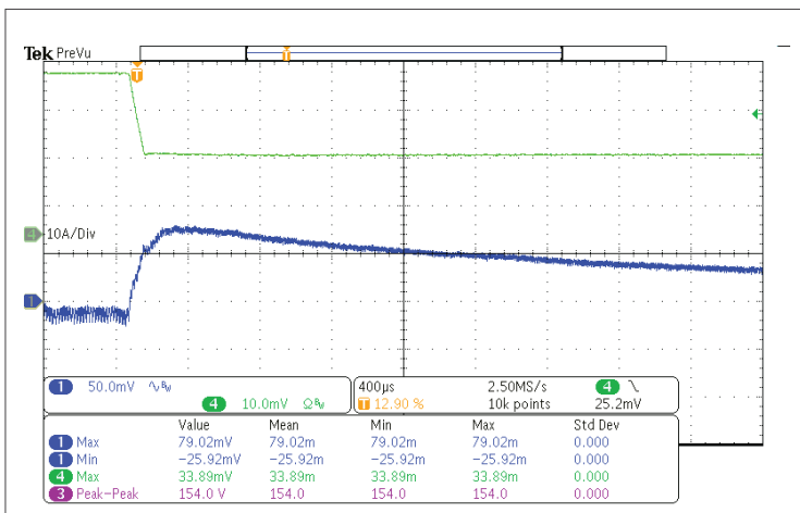
Fig. 36: TRANSIENT RESPONSE AT 115VAC, 50%-100% STEP LOAD.
