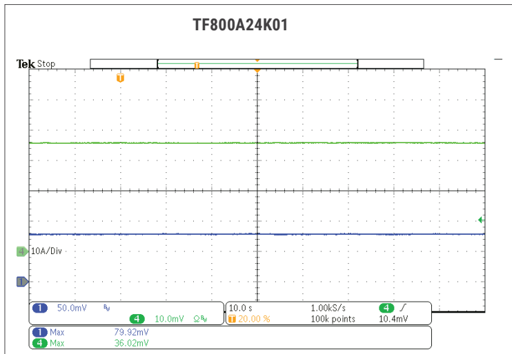
Fig. 22: SHORT CIRCUIT NO HCC-UP 115VAC.
