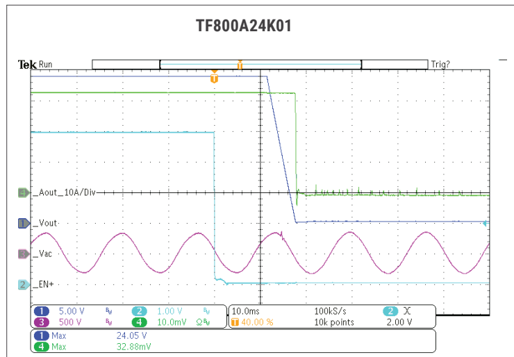
Fig. 57: INHIBIT (EN+)Lo Vout Off 230VAC.
