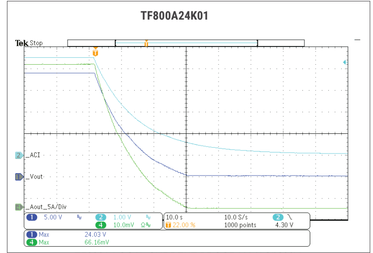
Fig. 45: LOCAL CURRENT PROGRAM (ACI) 230VAC.
