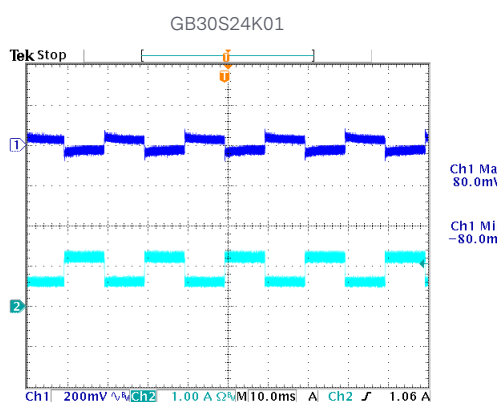
Fig. 56: TRANSIENT RESPONSE AT 230VAC, 50%-100% STEP LOAD. CH1: Vout, CH2: Load Current.
