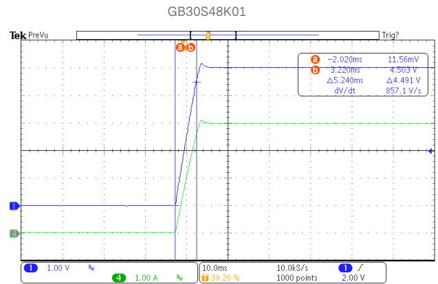
Fig. 26: TURN-ON RISE TIME AT 264VAC – 0.63A LOAD. CH1: Vout, CH4: Load Current.
