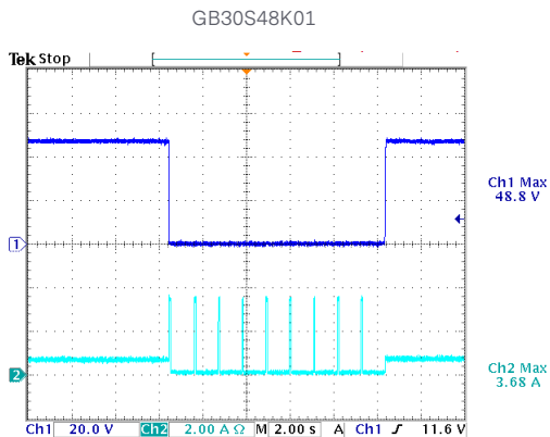
Fig. 49: OUTPUT SHORT CIRCUIT AT 115VAC. CH1: Vout, CH2: Short Circuit Current.
