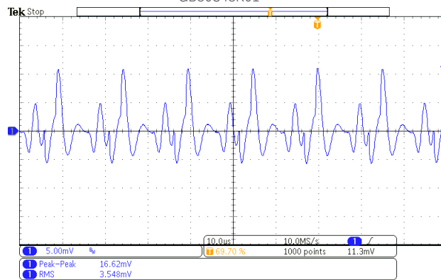
Fig. 66: COMMON MODE CURRENT AT 230VAC. CURRENT PROBE: 1mA/mV
