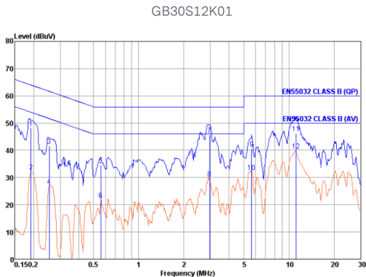
Fig. 73: EN55032 CLASS B – 230V/50Hz 100% LOAD MARGIN: >10 dB. Blue Plot: Quasi-Peak. Red Plot: Average.
