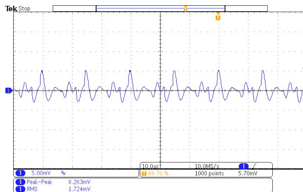
Fig. 64: COMMON MODE CURRENT AT 230VAC. CURRENT PROBE: 1mA/mV
