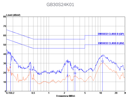
Fig. 76: EN55032 CLASS B – 120V/60Hz 10% LOAD MARGIN: >10 dB. Blue Plot: Quasi-Peak. Red Plot: Average.
