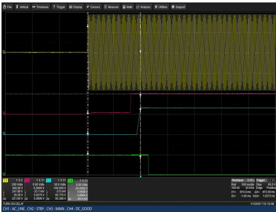
Figure 73: LCM30007-T Turn-on delay via AC mains Vin = 264Vac Load: Io = 41.7A (72V), Isb = 2A Ch 1: Vin Ch 2: Vsb Ch 3: Vo Ch 4: G_DCOK_C
