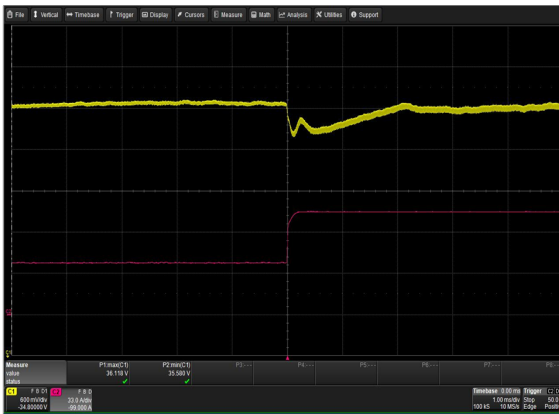
Figure 51: LCM3000U-T Transient Response - Vo Deviation 50% to 100% load change 1A/uS slew rate Vin = 230Vac Ch 1: Vo Ch 2: Io
