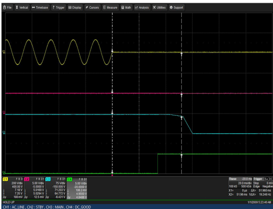
Figure 75: LCM30007-T Hold-up Time Vin = 90Vac Load: Io = 20.8A (72V), Isb = 2A Ch 1: Vin Ch 2: Vsb Ch 3: Vo Ch 4: G_DCOK_C
