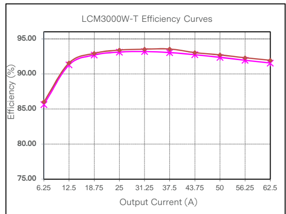
Figure 68: LCM3000W-T Efficiency Curve @ 25°C Loading: Io_min = 10%Io_max increment to 62.5A, Isb = 0A
