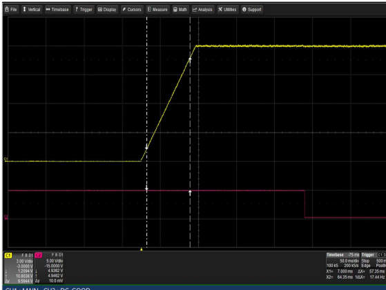
Figure 7: LCM3000L-T Output Voltage Startup Vin = 264Vac Load: Io = 125A (12V), Isb = 2A Ch 1: Vo Ch 2: G_DCOK_C
