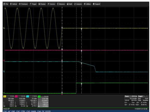
Figure 76: LCM30007-T Hold-up Time Vin = 264Vac Load: Io = 41.7A (72V), Isb = 2A Ch 1: Vin Ch 2: Vsb Ch 3: Vo Ch 4: G_DCOK_C
