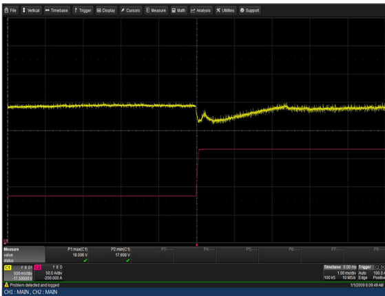
Figure 23: LCM30008-T Transient Response - V_o Deviation 50% to 100% load change 1A/ \mu s slew rate V_{in} = 230V_{ac} Ch 1: V_o Ch 2: I_o
