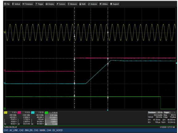
Figure 72: LCM30007-T Turn-on delay via INH_EN Vin = 90Vac Load: Io = 20.8A (72V), Isb = 2A Ch 1: Vin Ch 2: INH_EN Ch 3: Vo Ch 4: G_DCOK_C
