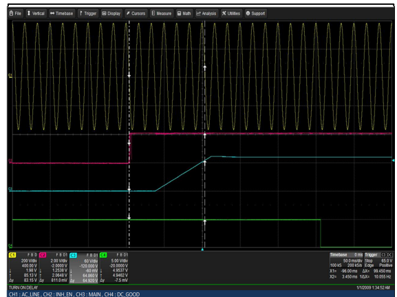
Figure 74: LCM30007-T Turn-on delay via INH_EN Vin = 264Vac Load: Io = 41.7A (72V), Isb = 2A Ch 1: Vin Ch 2: INH_EN Ch 3: Vo Ch 4: G_DCOK_C
