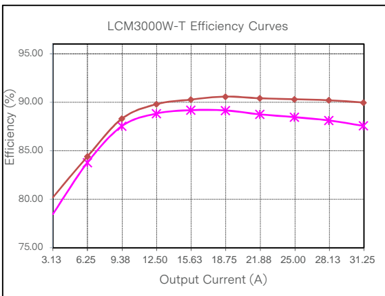
Figure 67: LCM3000W-T Efficiency Curve @ 25°C Loading: Io_min = 10%Io_max increment to 31.25A, Isb = 0A
