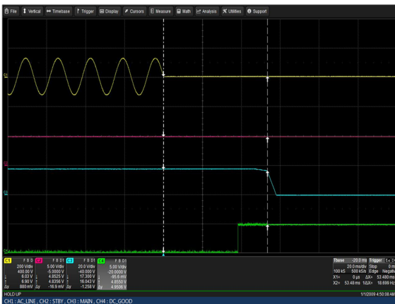
Figure 19: LCM30008-T Hold-up Time Vin = 90Vac Load: Io = 83.3A (18V), Isb = 2A Ch 1: Vin Ch 2: Vsb Ch 3: Vo Ch 4: G_DCOK_C
