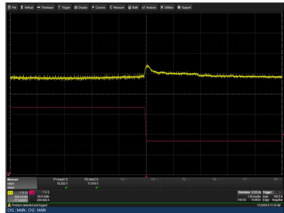
Figure 24: LCM30008-T Transient Response - V_o Deviation 100% to 50% load change 1A/ \mu s slew rate V_{in} = 230V_{ac} Ch 1: V_o Ch 2: I_o
