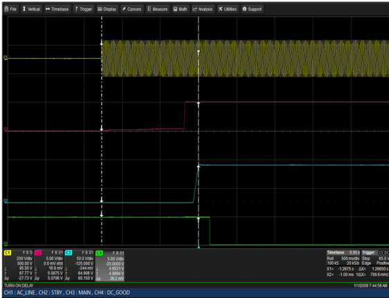
Figure 71: LCM30007-T Turn-on delay via AC mains Vin = 90Vac Load: Io = 20.8A (72V), Isb = 2A Ch 1: Vin Ch 2: Vsb Ch 3: Vo Ch 4: G_DCOK_C
