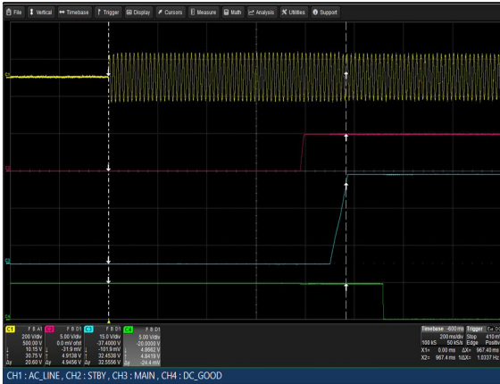
Figure 43: LCM3000U-T Turn-on delay via AC mains Vin = 90Vac Load: Io = 41.7A (36V), Isb = 2A Ch 1: Vin Ch 2: Vsb Ch 3: Vo Ch 4: G_DCOK_C
