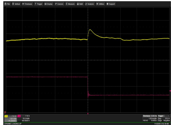
Figure 80: LCM30007-T Transient Response - Vo Deviation 100% to 50% load change 1A/μs slew rate Vin = 230Vac Ch 1: Vo Ch 2: Io
