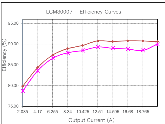
Figure 81: LCM30007-T Efficiency Curve @ 25°C Loading: Io_main = 10%Io_max increment to 20.8A, Isb = 0A — x — 90Vac — ◆ — 115Vac
