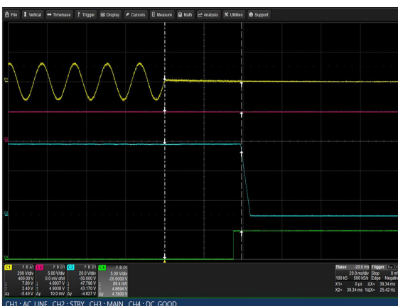
Figure 61: LCM3000W-T Hold-up Time Vin = 90Vac Load: Io = 31.25A (48V), Isb = 2A Ch 1: Vin Ch 2: Vsb Ch 3: Vo Ch 4: G_DCOK_C
