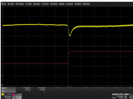
Figure 65: LCM3000W-T Transient Response - Vo Deviation 50% to 100% load change 1A/µs slew rate Vin = 230Vac Ch 1: Vo Ch 2: Io
