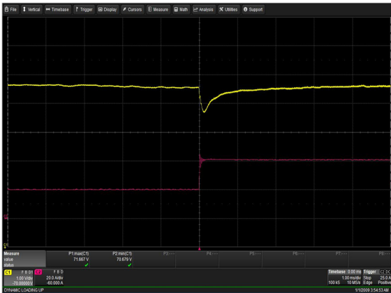
Figure 79: LCM30007-T Transient Response - Vo Deviation 50% to 100% load change 1A/μs slew rate Vin = 230Vac Ch 1: Vo Ch 2: Io
