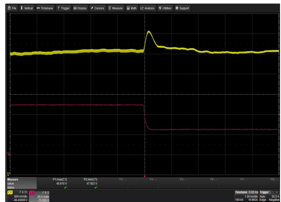
Figure 66: LCM3000W-T Transient Response - Vo Deviation 100% to 50% load change 1A/µs slew rate Vin = 230Vac Ch 1: Vo Ch 2: Io
