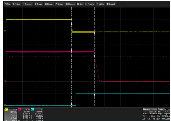
Figure 8: LCM3000L-T Turn Off Characteristic via INH_EN Vin = 264Vac Load: Io = 125A (12V), Isb = 2A Ch 1: INH_EN Ch 2: Vo Ch 3: G_DCOK_C
