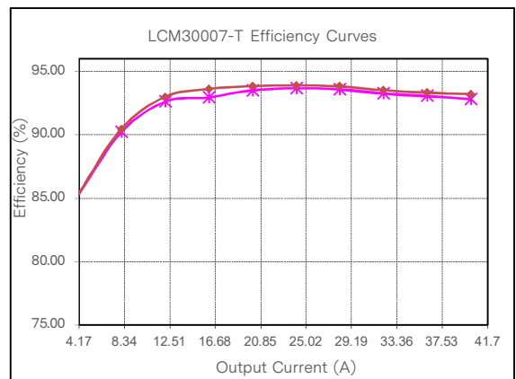
Figure 82: LCM30007-T Efficiency Curve @ 25°C Loading: Io_main = 10%Io_max increment to 41.7A, Isb = 0A — x — 230Vac — ◆ — 264Vac
