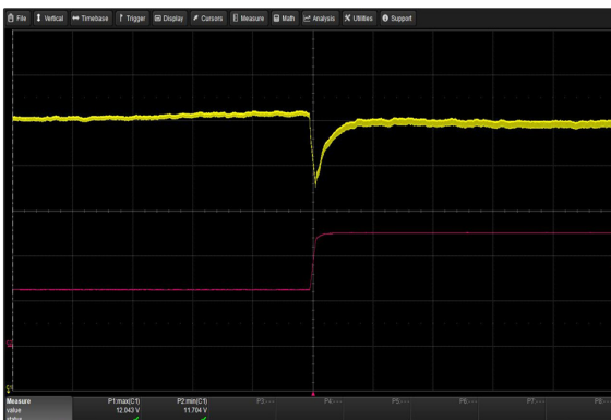
Figure 7: LCM3000L-T Output Voltage Startup Vin = 264Vac Load: Io = 125A (12V), Isb = 2A Ch 1: Vo Ch 2: G_DCOK_C
