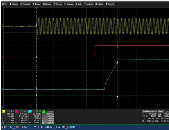
Figure 57: LCM3000W-T Turn-on delay via AC mains Vin = 90Vac Load: Io = 31.25A (48V), Isb = 2A Ch 1: Vin Ch 2: Vsb Ch 3: Vo Ch 4: G_DCOK_C
