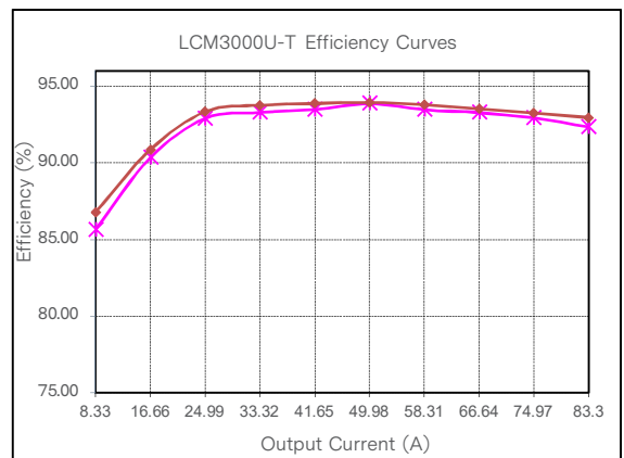
Figure 54: LCM3000U-T Efficiency Curve @ 25°C Loading: Io_main = 10%Io_max increment to 83.3A, Isb = 0A ◆ 230Vac ◆ 264Vac
