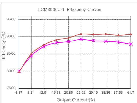
Figure 53: LCM3000U-T Efficiency Curve @ 25°C Loading: Io_main = 10%Io_max increment to 41.7A, Isb = 0A ◆ 90Vac ◆ 115Vac
