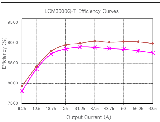
Figure 39: LCM3000Q-T Efficiency Curve @ 25°C Loading: Io_main = 10%Io_max increment to 62.5A, Isb = 0A
