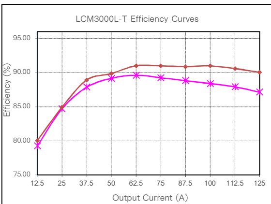
Figure 11: LCM3000L-T Efficiency Curve @ 25°C Loading: Io_main = 10%Io_max increment to 125A, Iss = 0A
