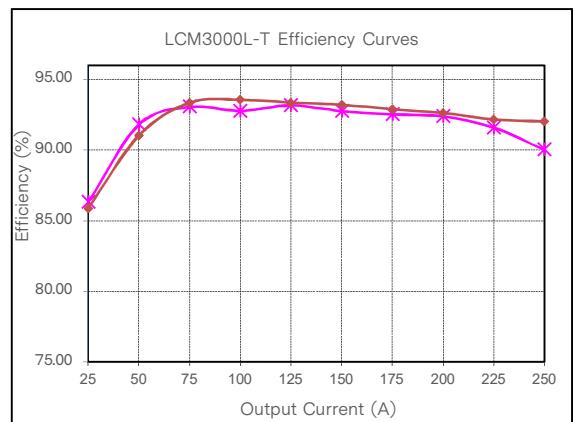
Figure 12: LCM3000L-T Efficiency Curve @ 25°C Loading: Io_main = 10%Io_max increment to 250A, Iss = 0A
