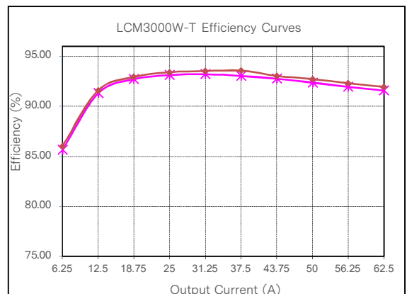
Figure 68: LCM3000W-T Efficiency Curve @ 25°C Loading: Io_main = 10%Io_max increment to 62.5A, Isb = 0A
