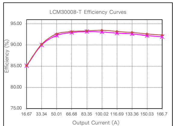
Figure 26: LCM30008-T Efficiency Curve @ 25°C Loading: Io_main = 10%Io_max increment to 166.7A, Isb = 0A
