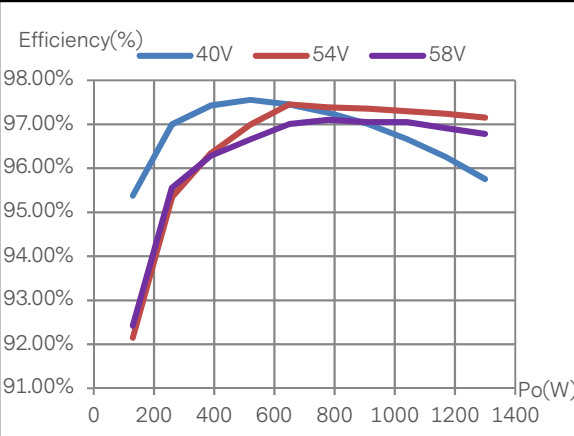
Figure 3: Efficiency vs Output Power T_A=25^\circ\text{C} , V_{IN}=40\text{V} , V_{IN}=54\text{V} , V_{IN}=58\text{V}
