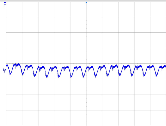
Figure 5: BDQ1300-48S12B-4L Input reflected Ripple Current Waveform Ch1: I_{IN} (10uS/div, 500mA/div) V_{IN}=54\text{V} , I_O=107\text{A}
