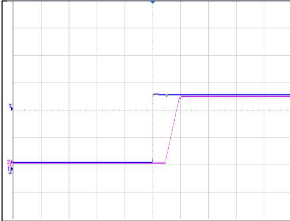
Figure 7: BDQ1300-48S12B-4L Output voltage startup by power on (50mS/div) V_{IN}=54V, I_O=107A Ch 1: V_{IN} (20V/div) Ch 2: V_O (5V/div)
