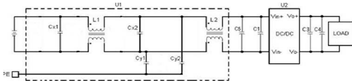
Figure 17 Typical application
