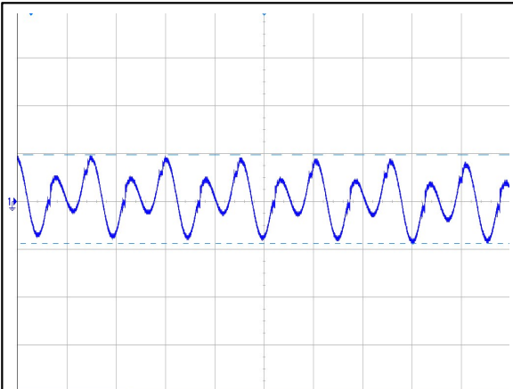
Figure 6: BDQ1300-48S12B-4L Ripple and Noise Measurement Ch1: V_O (5uS/div, 50mV/div) V_{IN}=54\text{V} , I_O=107\text{A}
