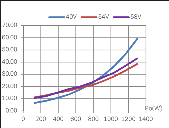
Figure 4: Power Loss vs Output Power T_A=25^\circ\text{C} , V_{IN}=40\text{V} , V_{IN}=54\text{V}
