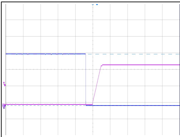
Figure 9: BDQ1300-48S12B-4L Output voltage startup by remote ON (50mS/div) V_{IN}=54V, I_O=107A Ch 1: Remote ON (1V/div) Ch 2: V_O (5V/div)
