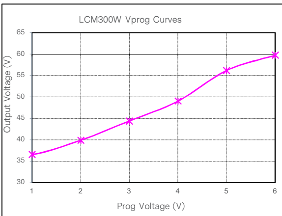
Figure 55: LCM300W Output Voltage Adjustment by Vprog @ 25°C Loading: I_o = 0A (48V), I_{SB} = 0A (5V)
