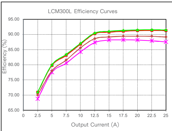
Figure 9: LCM300L Efficiency Curve @ 25°C — 90Vac — 115Vac — 230Vac — 264Vac Loading: I_{o\_main} = 10\%I_{o\_max} increment to 25A, I_{SB} = 0A (5V)
