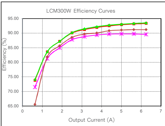
Figure 53: LCM300W Efficiency Curve @ 25°C Loading: I_{o\_main} = 10\%I_{o\_max} increment to 6.3A, I_{SB} = 0A (5V)
