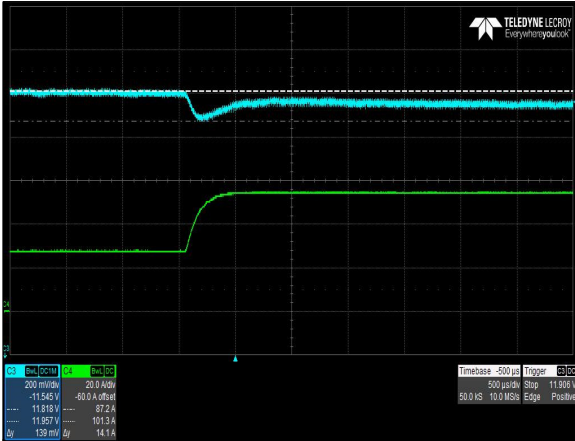
Figure 8: CNS653-ME Transient Response – Vo Deviation V_{IN} = 90\text{Vac} , I_O = 100\% to 50%, Output Cap = 330uF/A Ch 3: V_O Ch 4: I_O
