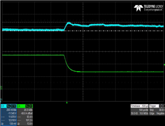
Figure 7: CNS653-ME Transient Response – Vo Deviation V_{IN} = 90\text{Vac} , I_O = 100\% to 50%, Output Cap = 330uF/A Ch 3: V_O Ch 4: I_O
