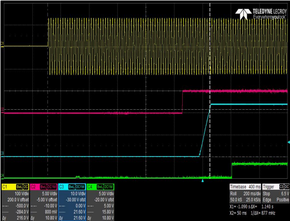
Figure 13: CNS655-MU Turn-on delay by AC Mains – Vin = 90Vac Load: I O = 16.7A, I SB = 1A Ch 1: V IN Ch 2: V SB Ch 3: V O Ch 4: PWOK
