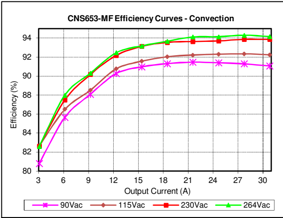
Figure 11: CNS653-MF Efficiency Curves @ 25°C Convection Cooling V_{IN} = 90 to 264Vac, Load: I_O = 0 to 30.8A
