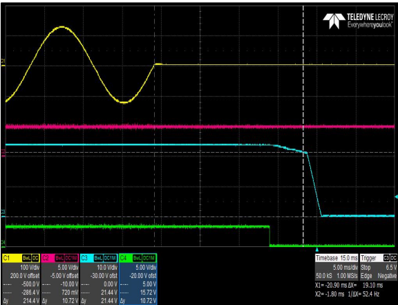
Figure 15: CNS655-MU Hold-up Time – Vin = 90Vac / 63Hz / 0° Load: I O = 16.7A, I SB = 1A Ch 1: V IN Ch 2: V SB Ch 3: V O Ch 4: PWOK
