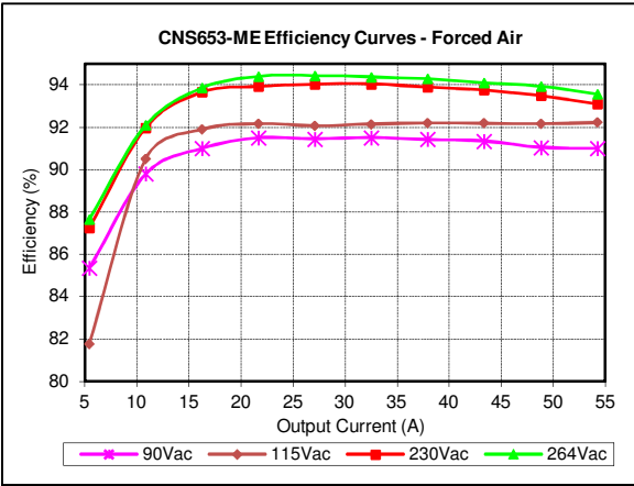
Figure 11: CNS653-ME Efficiency Curves @ 25°C Forced Air, Internal Fan V_{IN} = 90 to 264Vac, Load: I_O = 0 to 54.2A
