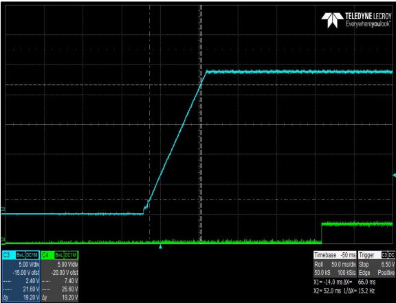
Figure 17: CNS655-MU Output Voltage Startup Characteristic Vin = 90Vac, Load: I O = 16.7A Ch 3: V O Ch 4: PWOK
