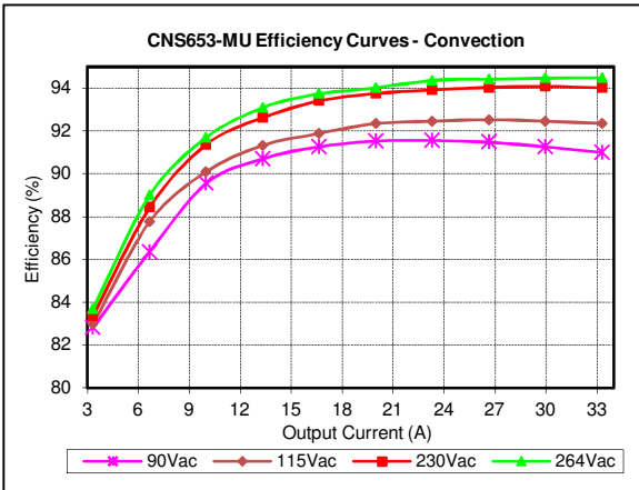
Figure 10: CNS653-MU Efficiency Curves @ 25°C Convection Cooling V_{IN} = 90 to 264Vac, Load: I_O = 0 to 33.3A
