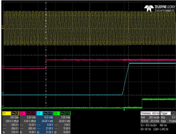
Figure 14: CNS655-MU Turn-on delay by Inhibit – Vin = 90Vac Load: I O = 16.7A, I SB = 1A Ch 1: V IN Ch 2: Inhibit Ch 3: V O Ch 4: PWOK
