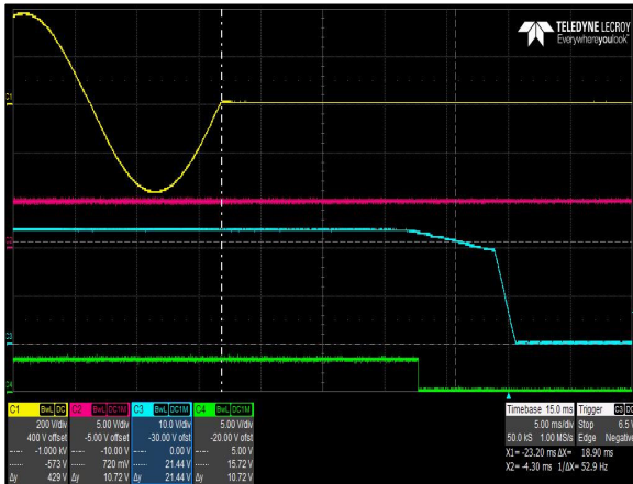
Figure 16: CNS655-MU Hold-up Time – Vin = 264Vac / 47Hz / 0° Load: I O = 16.7A, I SB = 1A Ch 1: V IN Ch 2: V SB Ch 3: V O Ch 4: PWOK
