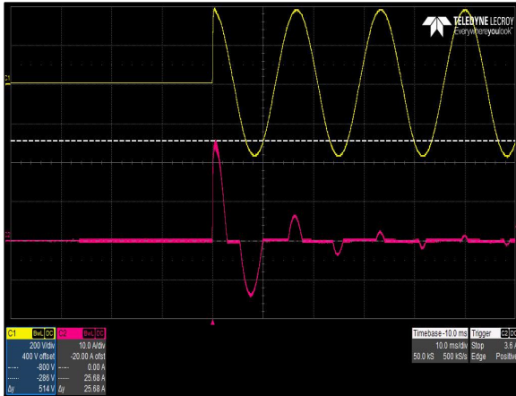
Figure 18: CNS655-MU Inrush Current V IN = 264Vac, Load: I O = 0A, Turn on angle = 90° Ch 1: V IN Ch 2: I IN
