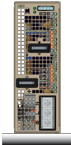
MOUNTING "A"
