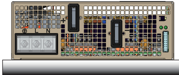
MOUNTING "B"
