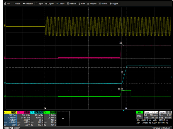
Figure 2: LCC1200-28U-9P Turn-on delay via AC mains Vin = 264Vac Load: Io = 42.9A (28V), I SB = 1.5A (5V) Ch 1: AC Mains Ch 2: V SB Ch 3: V O CH 4: G_DCOK_C
