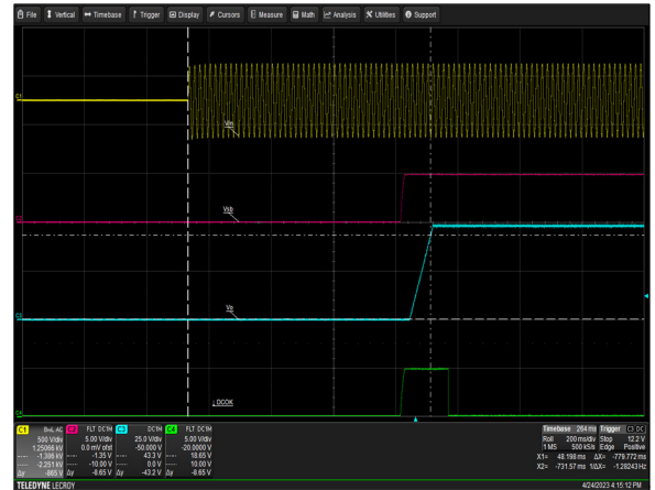
Figure 14: LCC1200-48U-9P Turn-on delay via AC mains Vin = 264Vac Load: Io = 25A (48V), I SB = 1.5A (5V) Ch 1: AC Mains Ch 2: V SB Ch 3: V 0 CH 4: G_DCOK_C
