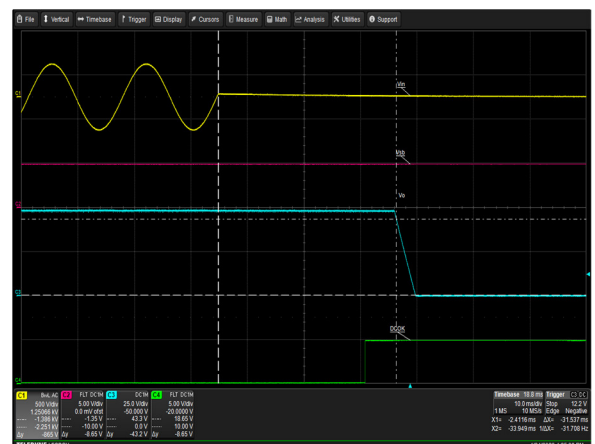
Figure 18: LCC1200-48U-9P Hold-up Time Vin = 264Vac Load: Io = 25A (48V), I SB = 1.5A (5V) Ch 1: AC Mains Ch 2: V SB Ch 3: V 0 CH 4: G_DCOK_C
